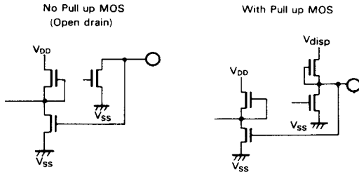
Figure 17 I/O Configuration
