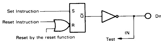
Figure 15 1-bit Discrete I/O Block Diagram
