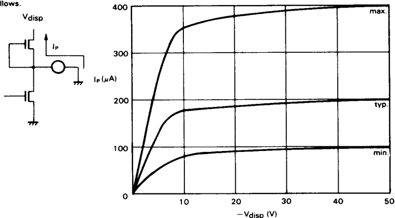
Figure 1 I_p vs. V_{disp}
