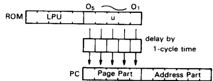
Figure 8 LPU Operation
